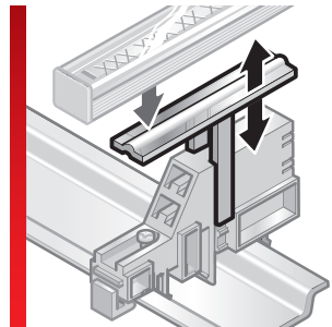
Terminal socket with indicator
