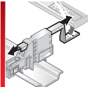
Terminal socket with spacer block
