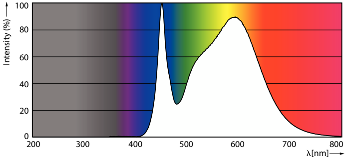
Spectral Power Distribution Colour - CorePro LED PLC 8.9W 840 2P G24d-3
