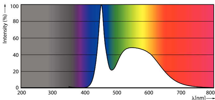
Spectral Power Distribution Colour - Ecofit LEDtube 1500mm HO 23W 865 T8 S
