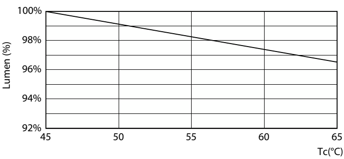
Lumen Maintenance Diagram - CorePro LEDtube HF 1200mm HE 17.1W 840T5
