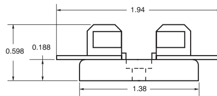
4520 integral clip and straight solder terminals
