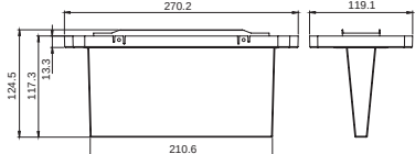
Cone diffuser - Dimensional drawings (mm)
