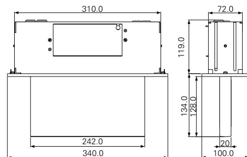
1803 LED CG-S
