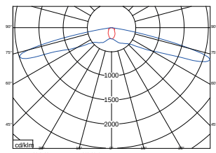
Light distribution curve HandRail 930x1 LED
