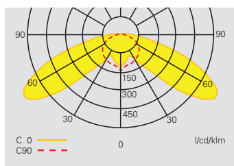
Light distribution curve FlexiTech SE 400 CG-S
