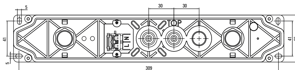
Dimensions in mm (quick-mounting set)
