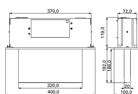
1804 LED CG-S
