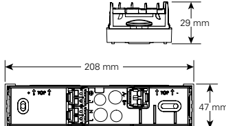
Add-on housing
