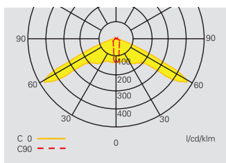
Light distribution curve Atlantic LED II R CG-S with asymmetric optics
