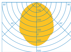
Light distribution curve BeamTech wide beam
