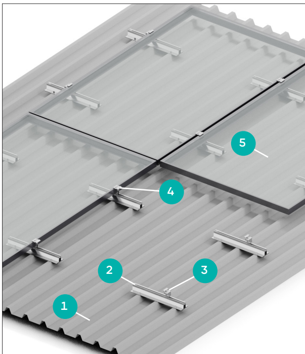
Image 2.1. - 1 Portrait Installation
