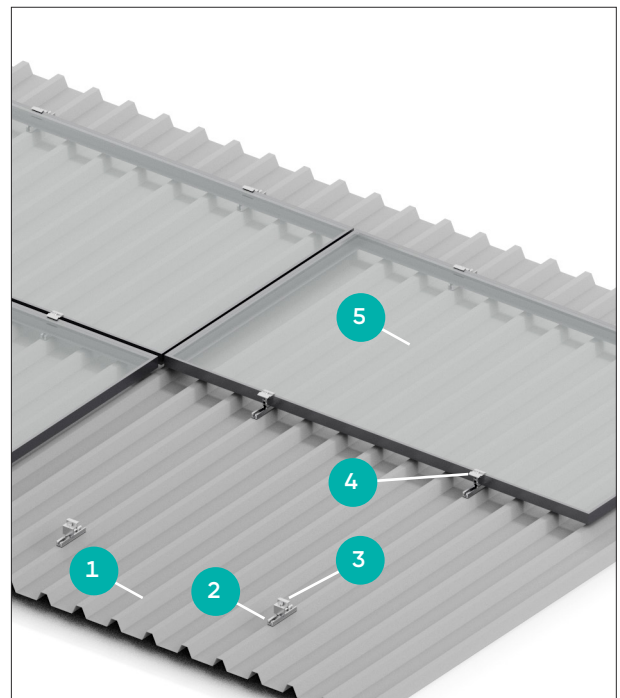
Image 2.1. - 2 Landscape Installation
