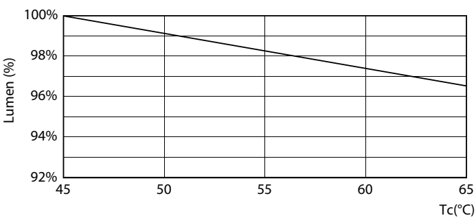
Lumen Maintenance Diagram - CorePro LEDtube HF 1500mm HO 26.7W 830T5
