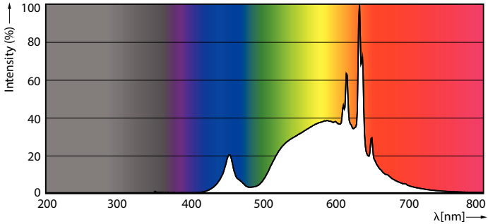
Spectral Power Distribution Colour - MAS LEDBulb D 4-60W E27 830 A60 FR G UE
