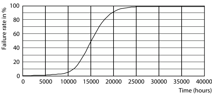
Life Expectancy Diagram - CorePro LEDBulbND 150W E27 A67 840 CL G
