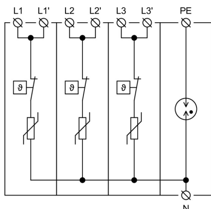
Internal diagram
