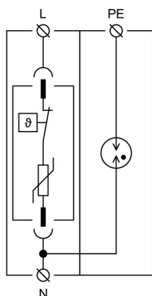
Internal diagram
