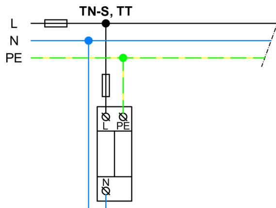
Application wiring diagram (installation)
