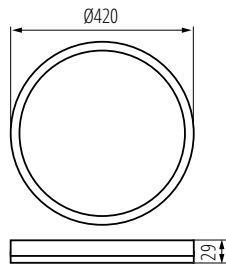
AZPO LED 22W-O
