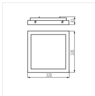
TYBIA LED 25W
